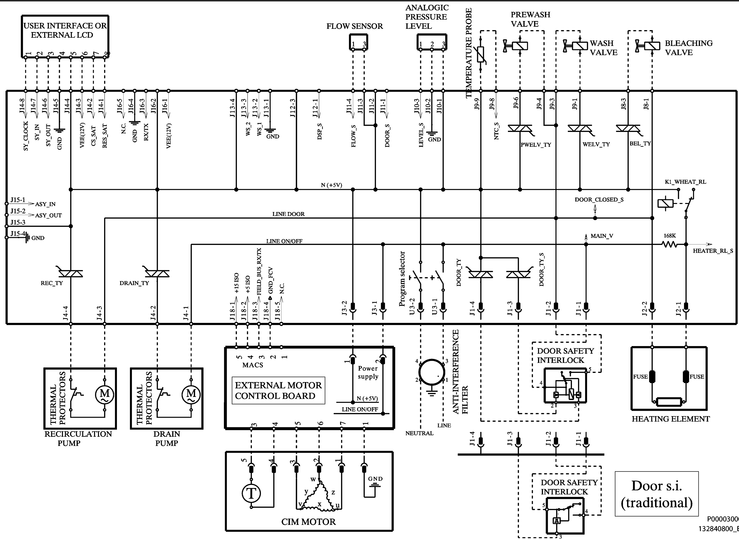
ELECTRIC DIAGRAM -
