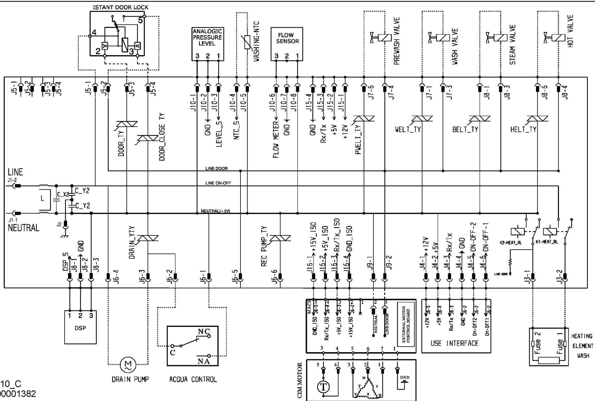
ELECTRIC DIAGRAM EWM10
