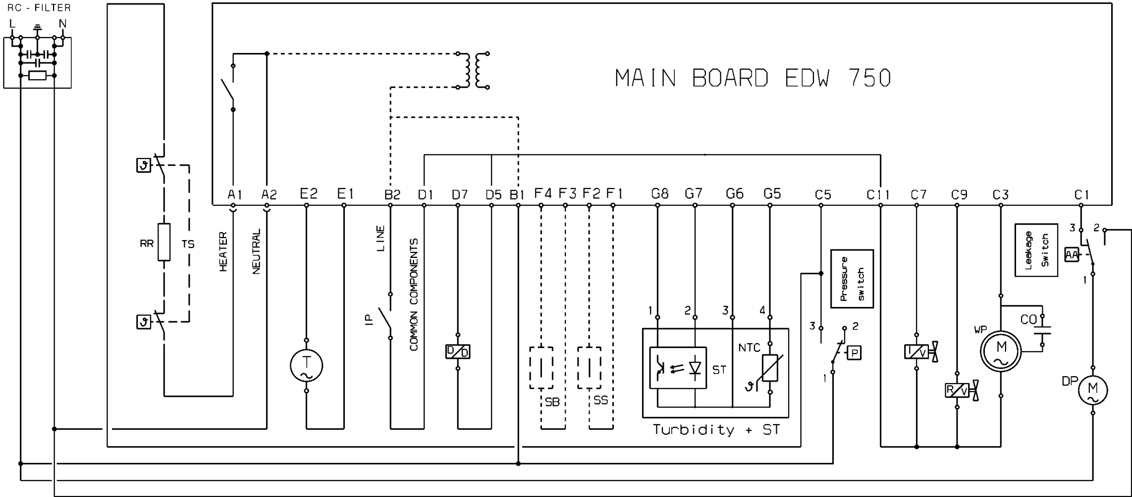
CIRCUIT DIAGRAM
