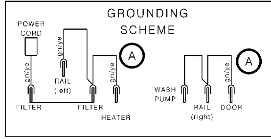
Connections included in WireHarnesses
