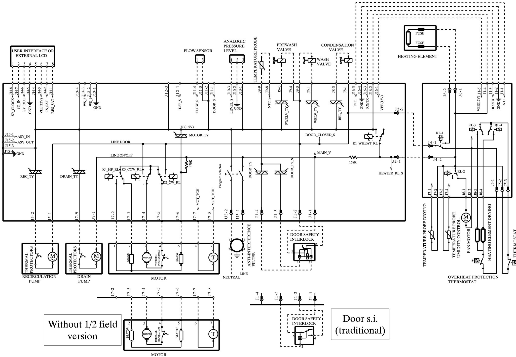
ELECTRIC DIAGRAM
