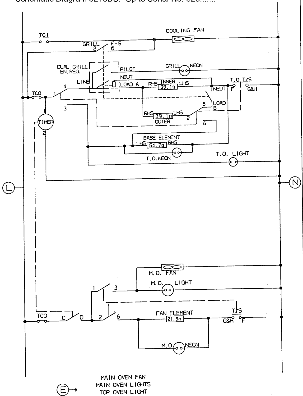
Schematic Diagram 3210BU. Up to Serial No. 823.....
