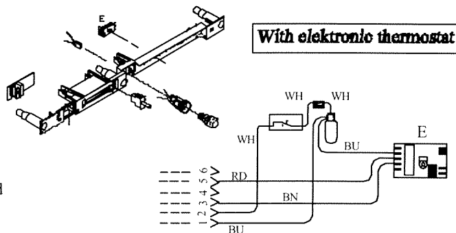
Terminal board
