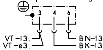
h1 Gluehlampe
