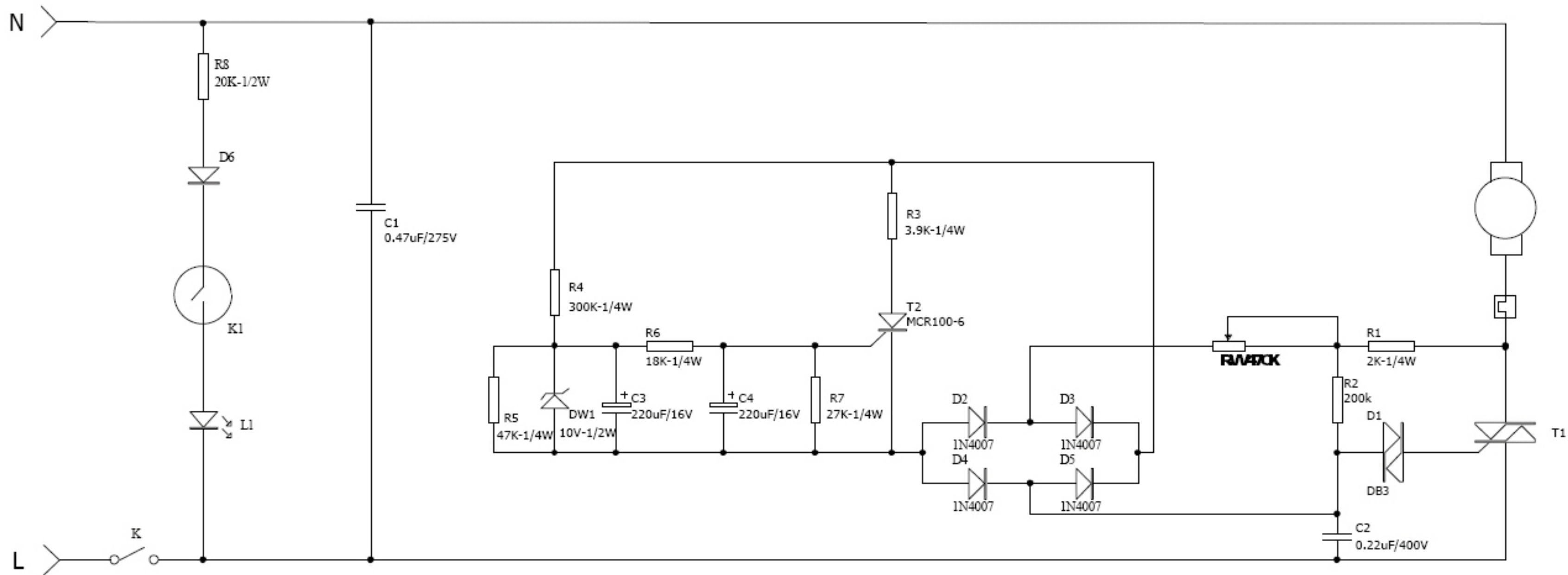
WIRING DIAGRAM 73series
