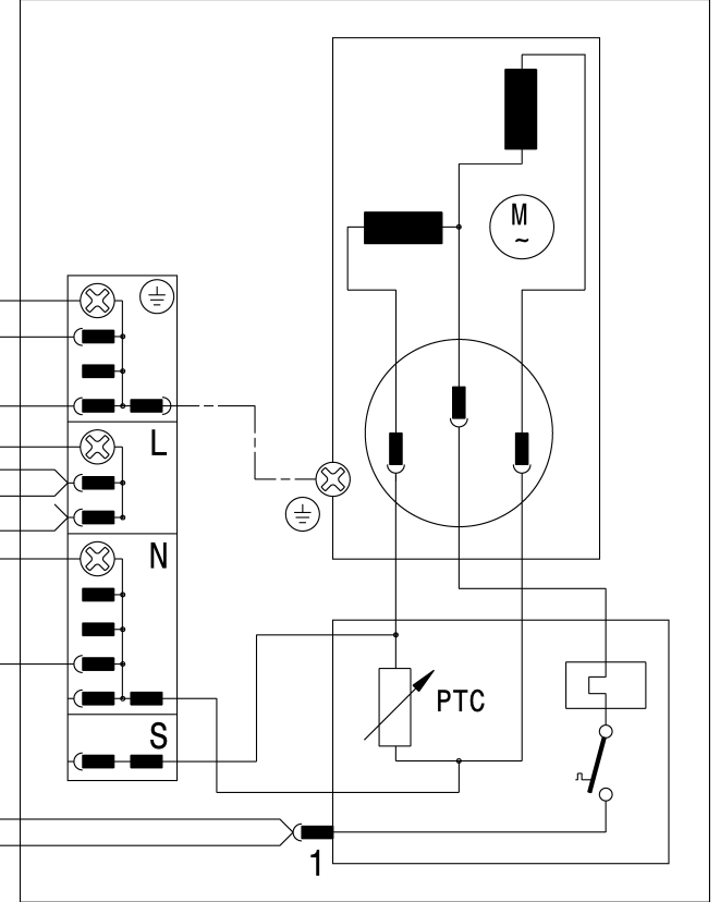
Compressor
