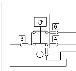
Thermostat
