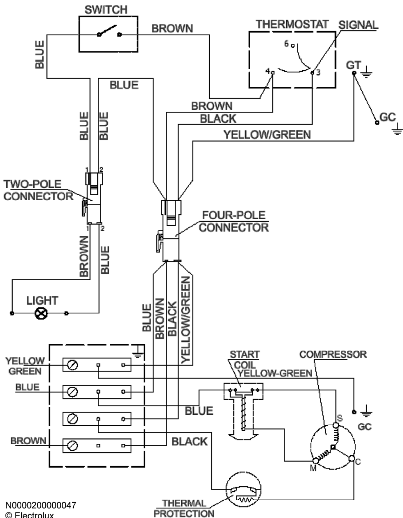
Electric diagram for compressors type S, GQR, AES and GQT
